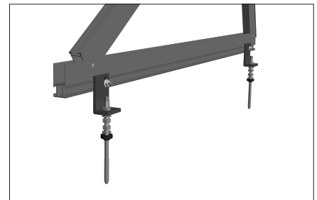
Adapter for hanger bolts
