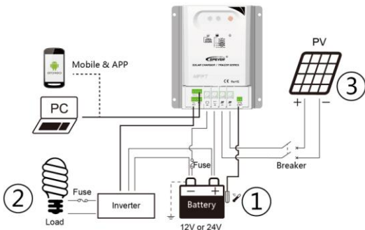
Figure 2-1 Mounting
